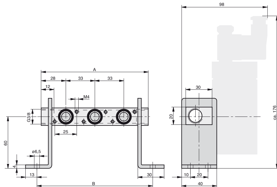
P-Manifold with long mounting brackets Type: PL-1/4-...
