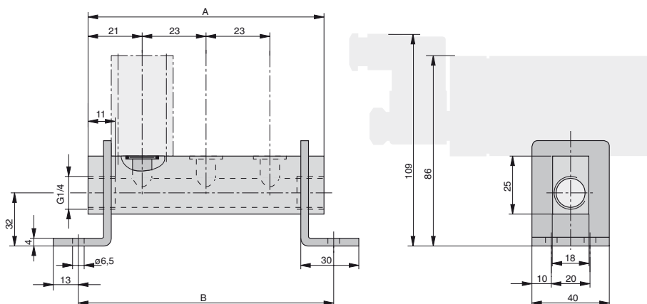
P-Supply Manifold with short mounting brackets Type: PLK-1/8-..
