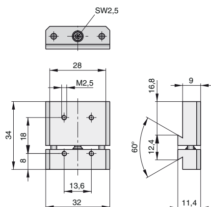
Dimension Table – Adapter Plate for Single Valves S10-1/8 (Q6)
