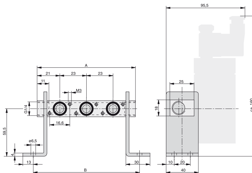
P-Manifold with long mounting brackets Type: PL-1/8-..
