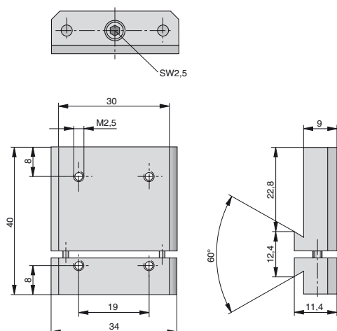
Dimension Table – Adapter Plate for Single Valves S10-1/4 (Q8)
