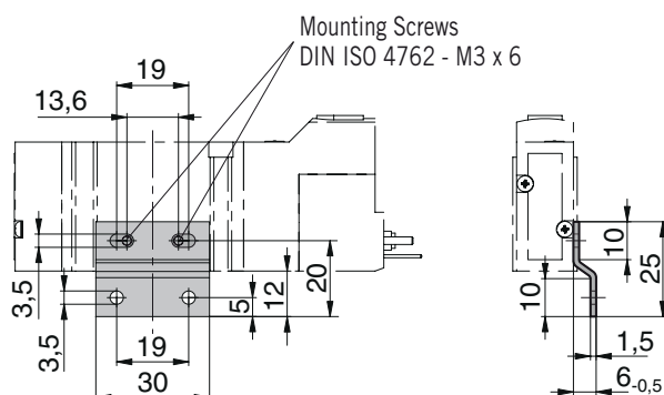
Dimension Table – Mounting Bracket for Single Valves
