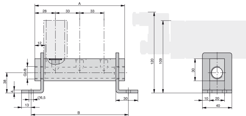
P-Manifold with short mounting brackets Type: PLK-1/4-...
